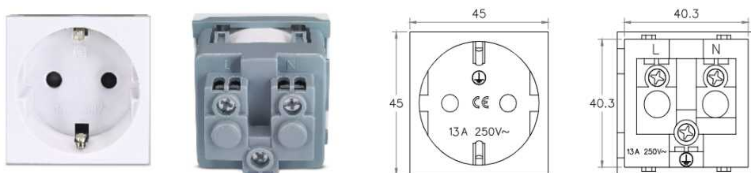
MX 7254 3 Pin French Socket W/Shutter 2 Module 13A/250V White
