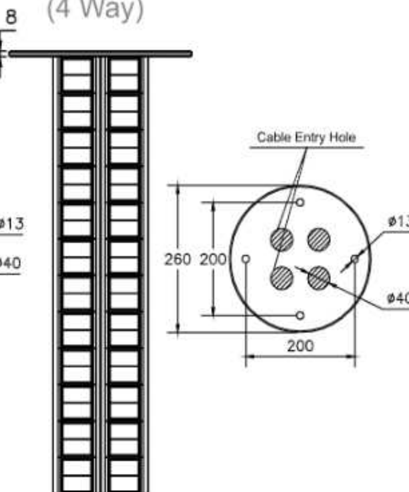
MX 6420 CM (4 Way)
