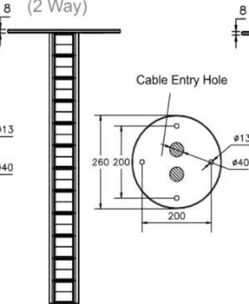
MX 6419 CM (2 Way)
