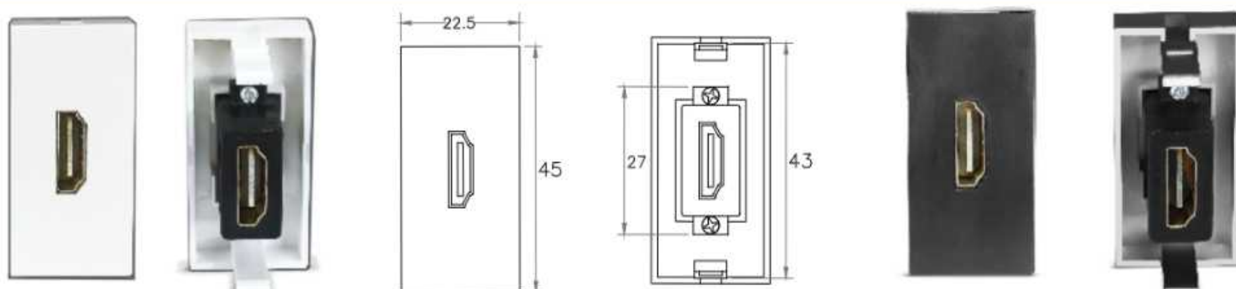
MX 7256 White HDMI To HDMI Connector 1 Module MX 7257 Black
