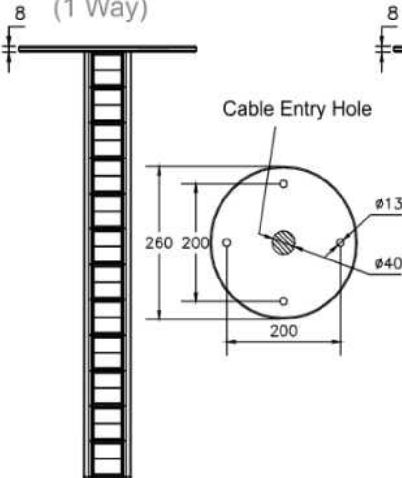
MX 6418 CM (1 Way)
